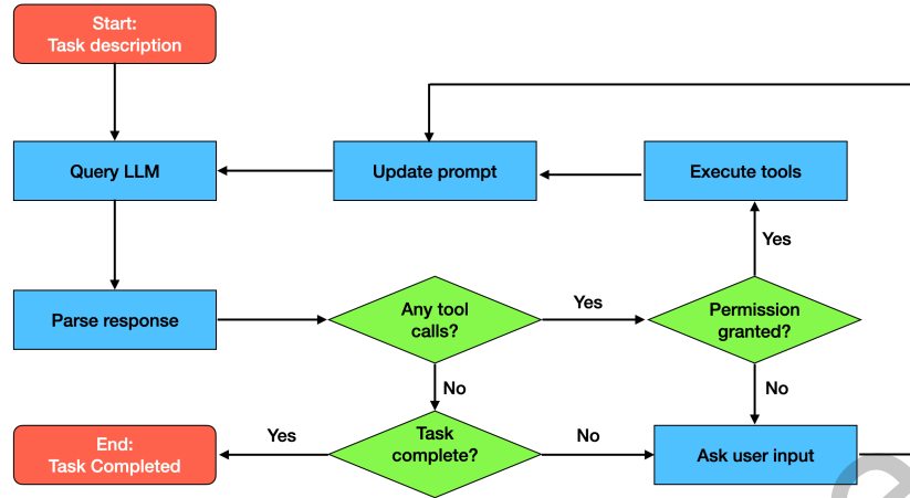
Fig. 1. Typical workflow of a coding agent
